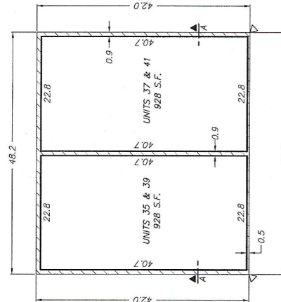
BASEMENT PLAN ALL EXTERIOR WALLS ARE .9 THICK (UNLESS OTHERWISE NOTED)
