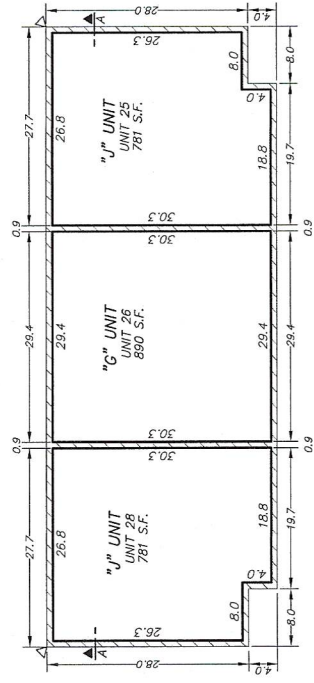
BASEMENT PLAN
