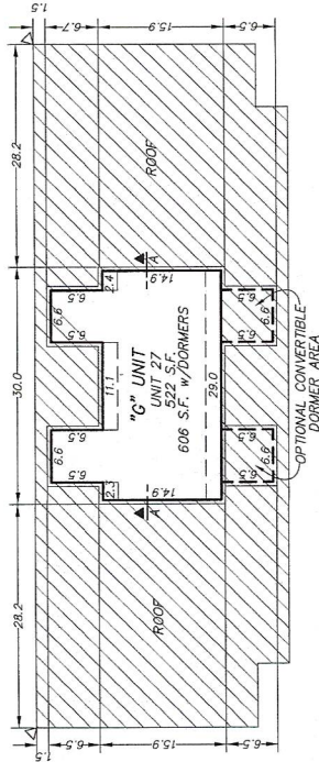
ATTIC SPACE PLAN
